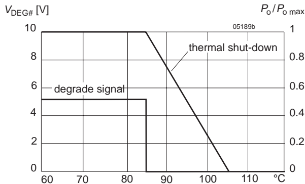
Fig. 9 Degrade signal V_{\text{DEG}\#} versus case temperature T_C
